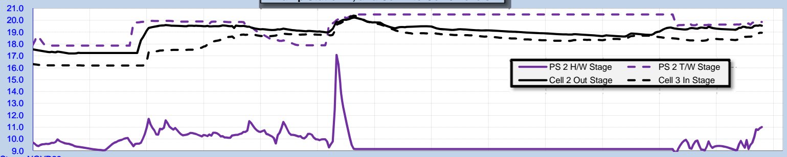
Pump Station 2, and Cell 2 to Cell 3 Levels
